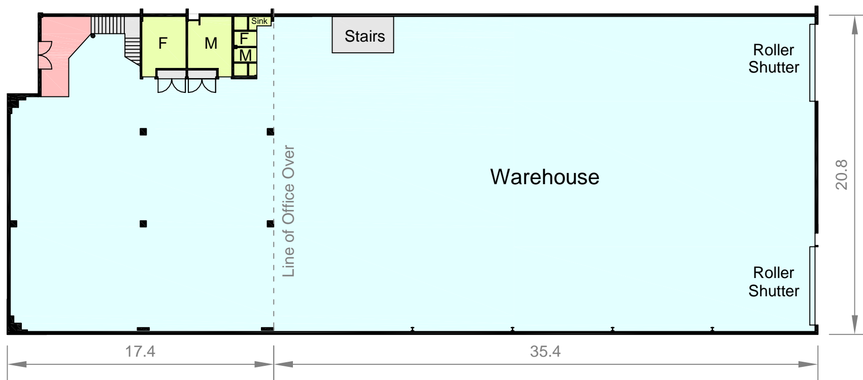
GROUND FLOOR
